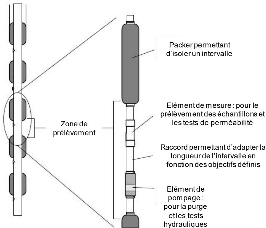
Figure 21 : Système Westbay (source: Practical Handbook of environmental site characterization and ground-water monitoring , 2005)
