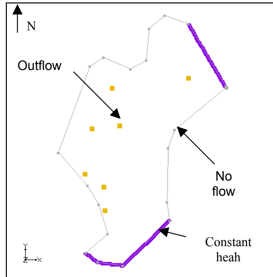
Figure 3 : Modelled domain and boundary conditions
