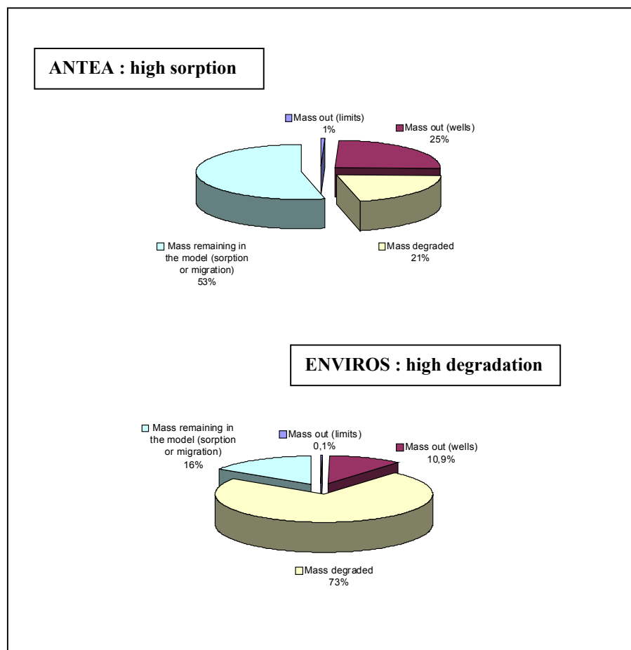
Figure 6 : Comparison between ANTEA and ENVIROS PCE mass balance (kg) (0 to 1800 days)
